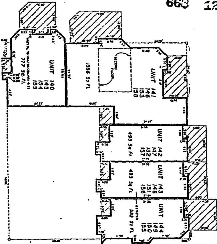
FIRST FLOOR PLAN - BUILDING (K, L, M, N)
